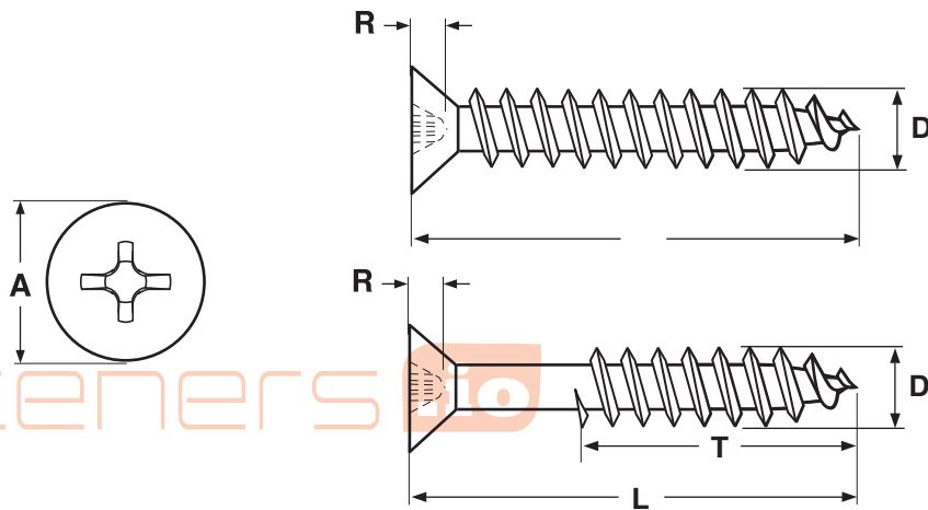
FLAT PHILLIPS DEEP THREAD WOOD SCREW
