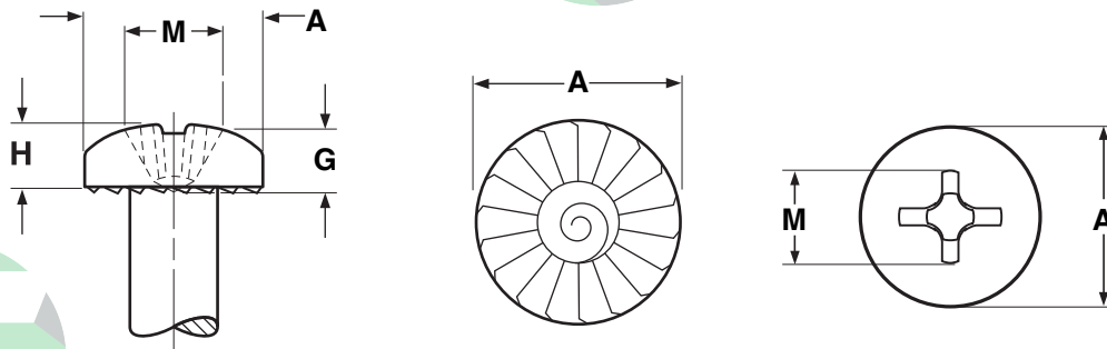
SERRATED PAN PHILLIPS FOR TAPPING SCREWS
