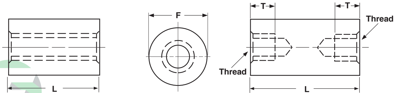
ROUND STANDOFFS
