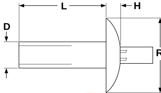
BRAZIER HEAD DRIVE PIN RIVETS
