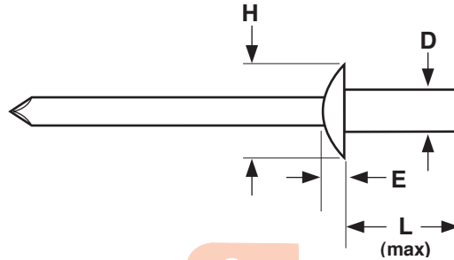
CLOSED-END, DOME HEAD, ALUMINUM BODY/STEEL MANDREL BLIND RIVETS
