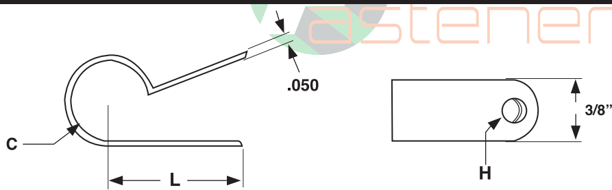
NYLON STANDARD CABLE CLAMPS—3/8" WIDE CONTACT AREA
