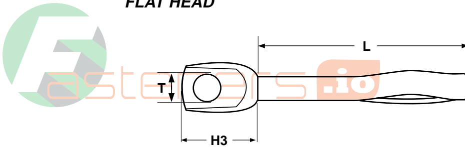
TIE-WIRE HEAD
